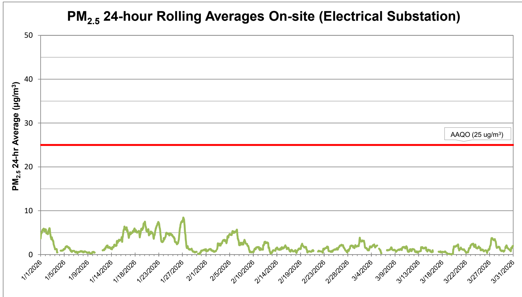
Figure 1: 24-hour rolling averages of PM 2.5 data from on-site monitor for the first calendar quarter 2026 (January 1 st to March 31 st , 2026)
