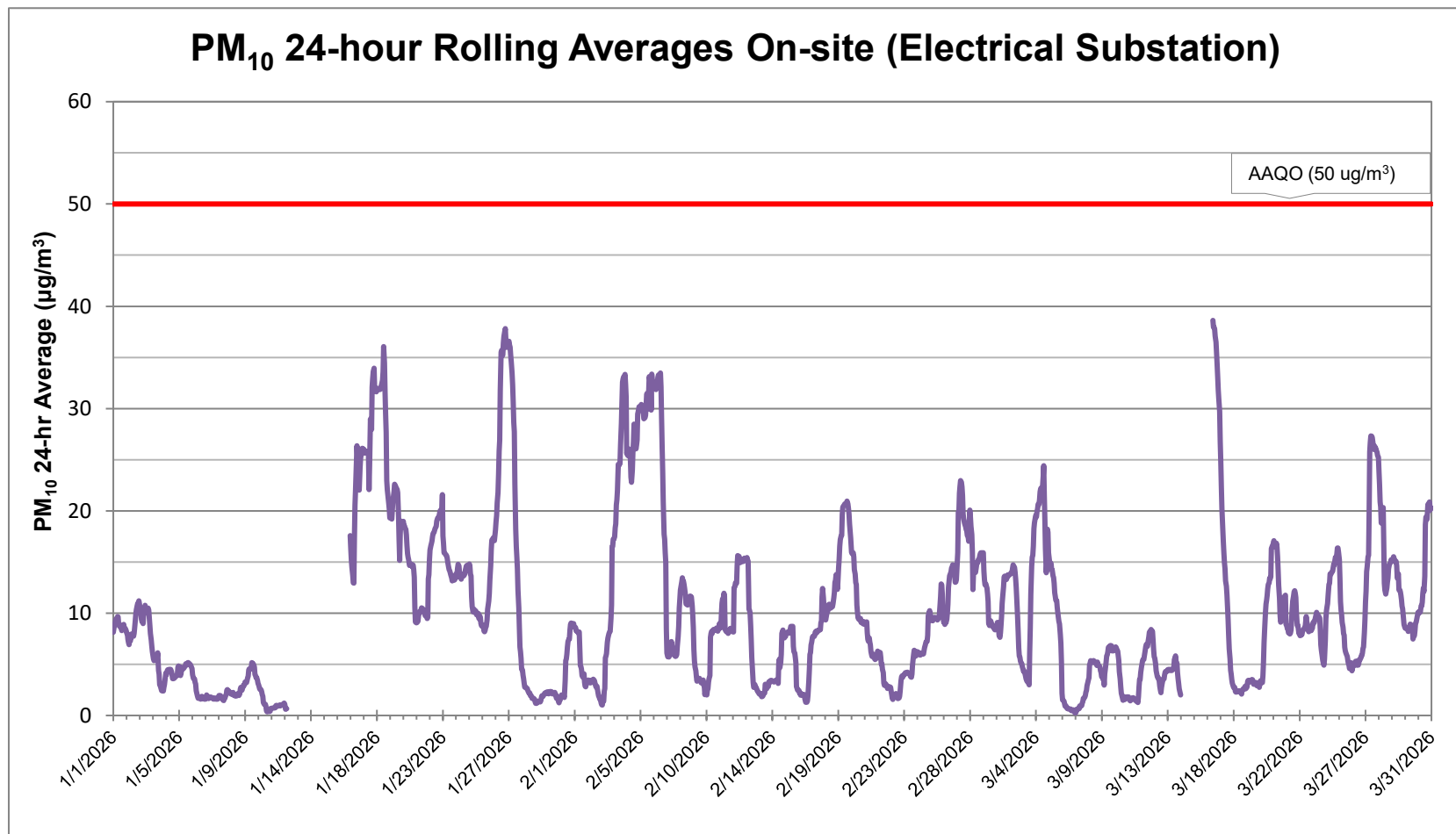
Figure 2: 24-hour rolling averages of PM 10 data from on-site monitor for the first calendar quarter 2026 (January 1 st to March 31 st , 2026)
