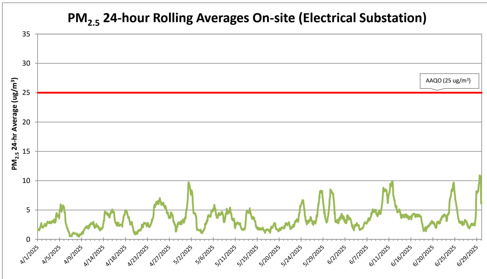
Figure 1: 24-hour rolling averages of PM 2.5 data from on-site monitor for the second calendar quarter 2025 (April 1 st to June 30 th , 2025)
