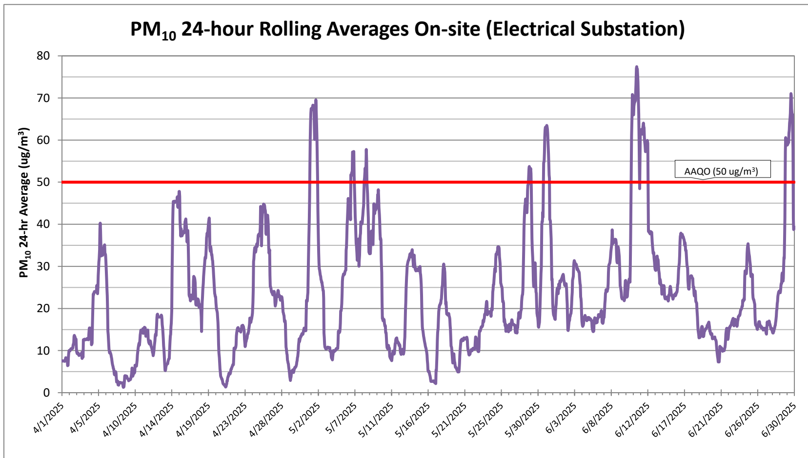
Figure 2: 24-hour rolling averages of PM 10 data from on-site monitor for the second calendar quarter 2025 (April 1 st to June 30 th , 2025)
