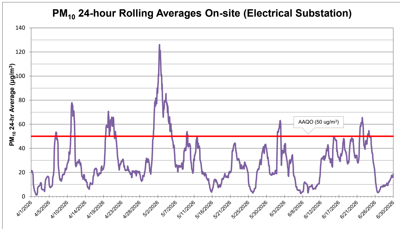
Figure 2: 24-hour rolling averages of PM 10 data from on-site monitor for the second calendar quarter 2026 (April 1 st to June 30 th , 2026)
