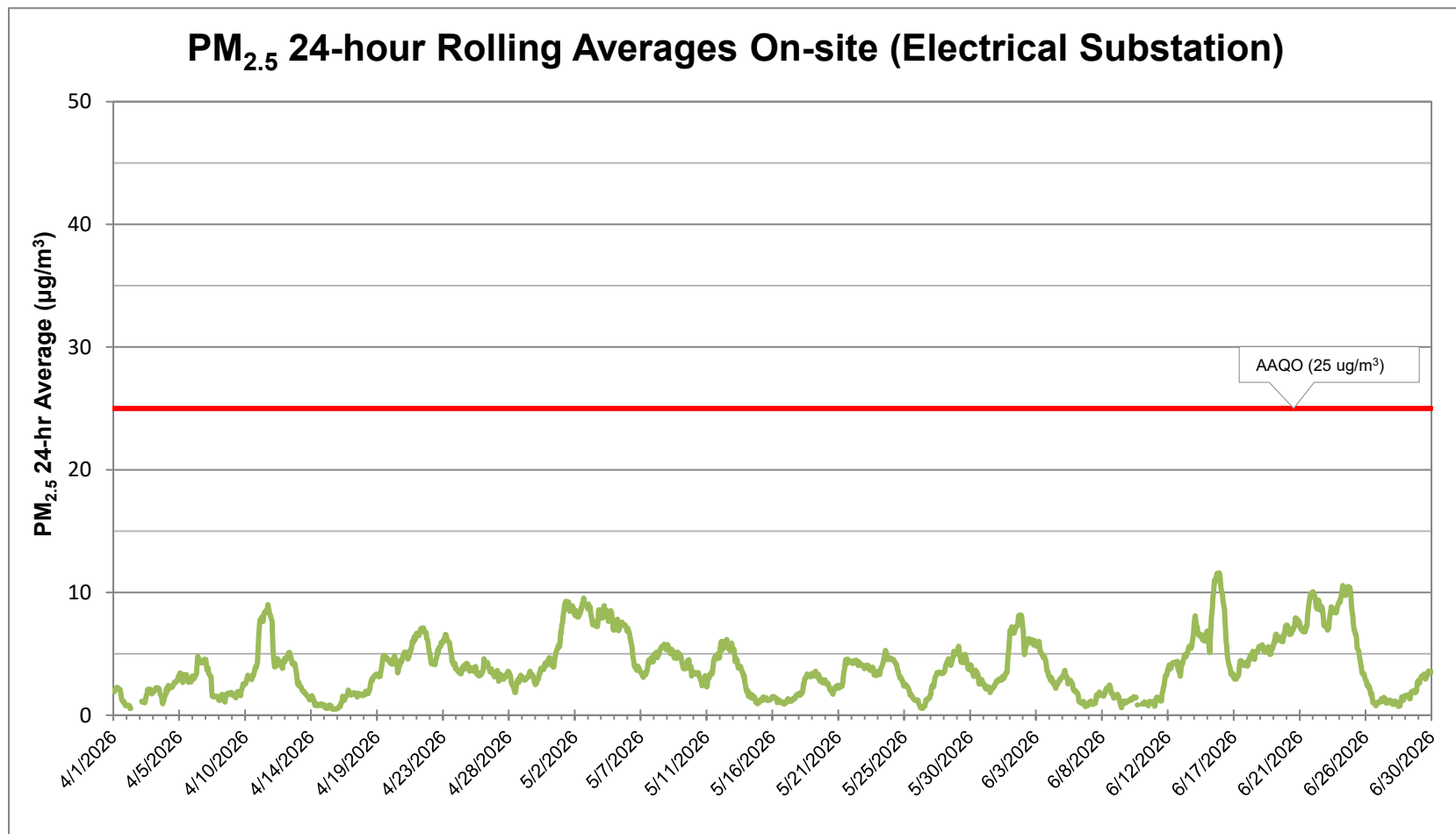
Figure 1: 24-hour rolling averages of PM 2.5 data from on-site monitor for the second calendar quarter 2026 (April 1 st to June 30 th , 2026)
